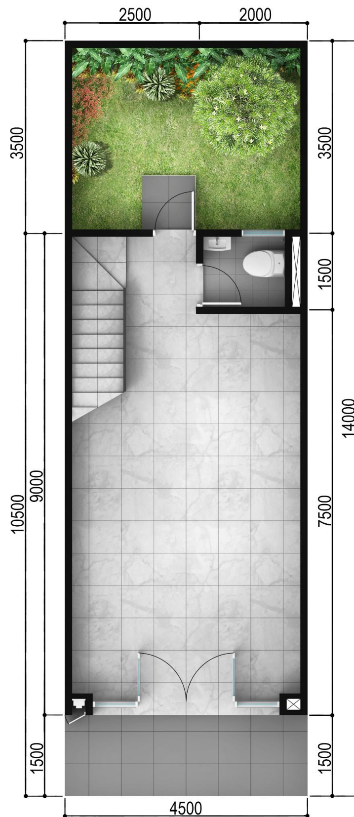
DENAH LANTAI 1
