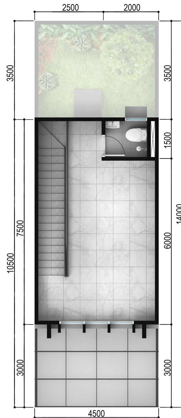
DENAH LANTAI 3
