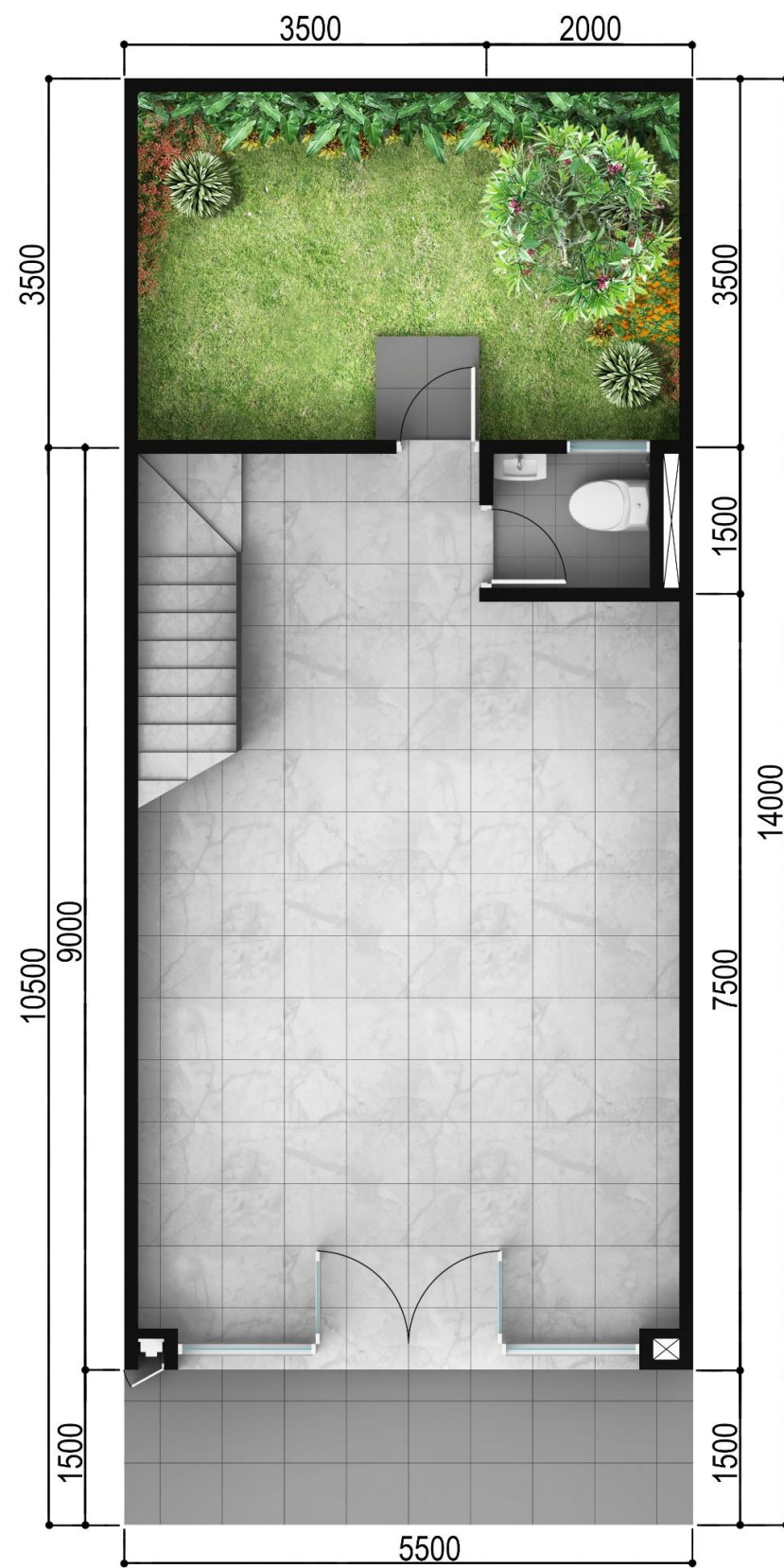
DENAH LANTAI 1
