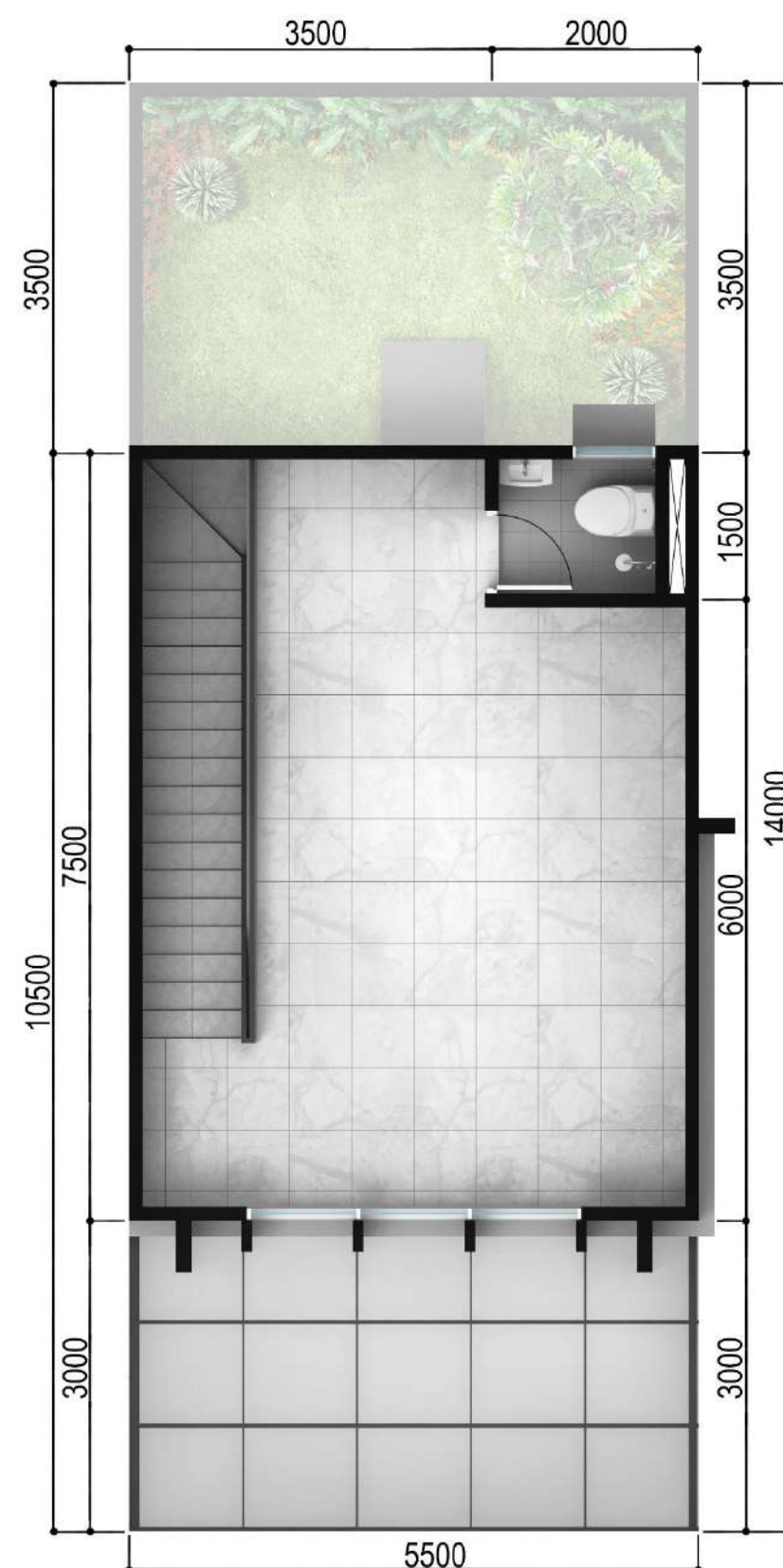
DENAH LANTAI 3
