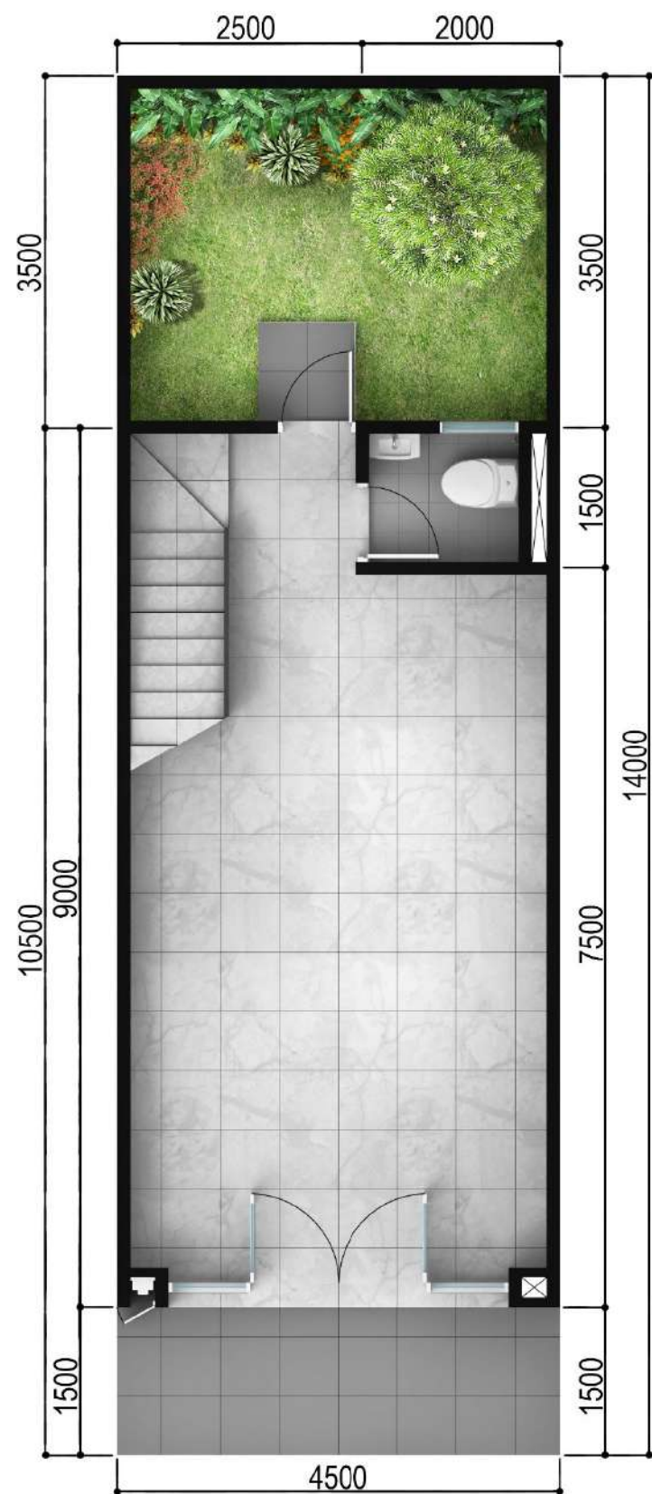
DENAH LANTAI 1
